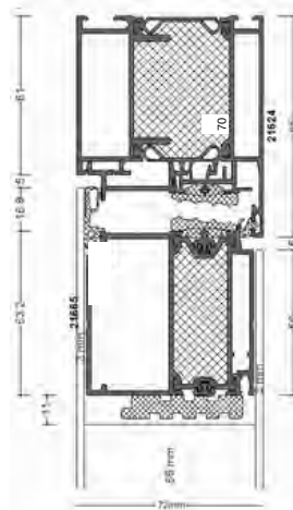
Frame/Sash section detail
